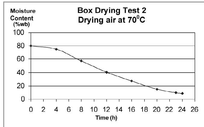
Figure 2: Typical drying curve when drying at 70°C
