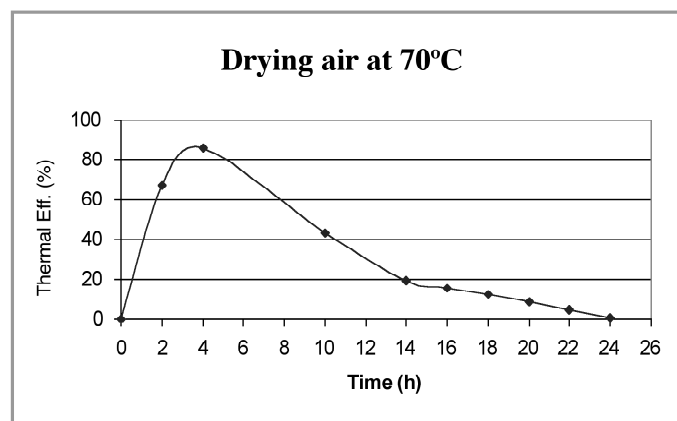
Figure 4: Thermal Efficiency curve when drying at 70°C
