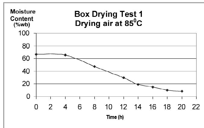
Figure 1: Typical drying curve when drying at 85°C
