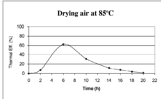
Figure 3: Thermal Efficiency curve when drying at 85°C
